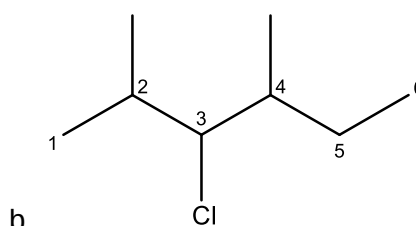
3-chloro-2,4-dimethylhexane
