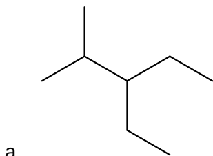
3-ethyl-2-methylpentane
